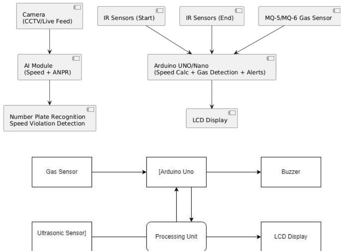
Fig: Proposed System Architecture
